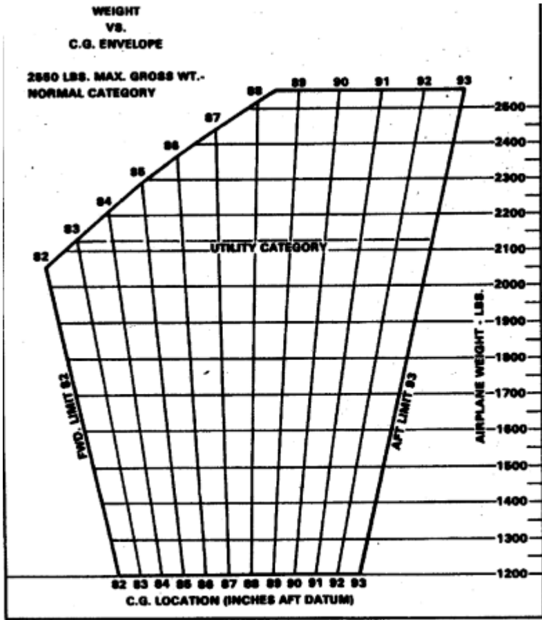
C.G. RANGE AND WEIGHT Figure 6-15
